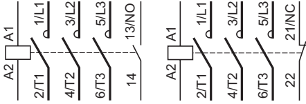
LC1E06...38
