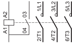
LC1E400, 500, 630
