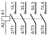
LC1E06...95004
