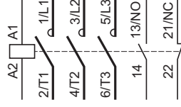
LC1E40...95
